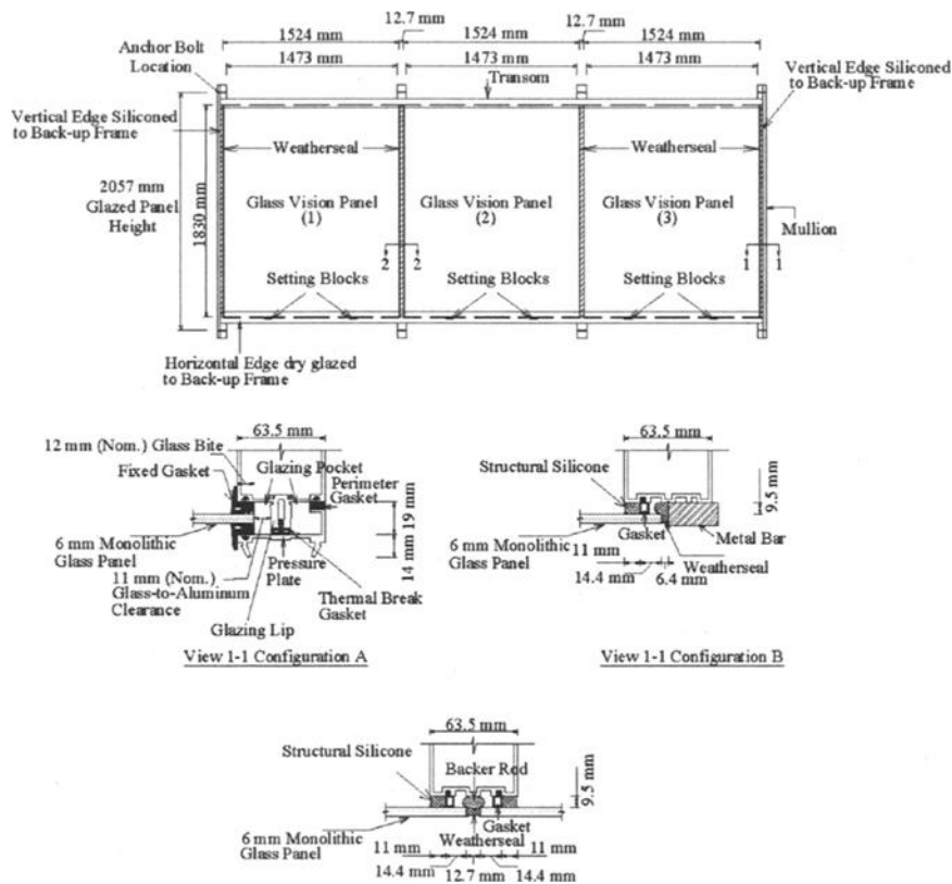
FIG. 1—Glazing details of Configurations A and B (1 mm=0.0394 in.)
