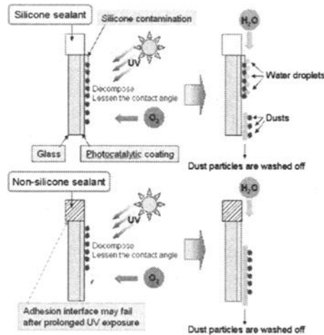
FIG. 1—Cleaning mechanism of SCG.
