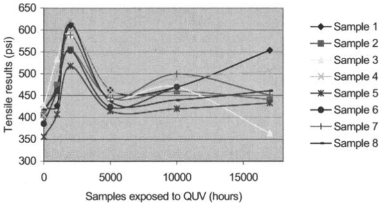
FIG. 1— Tensile strength versus QUV exposure time.
