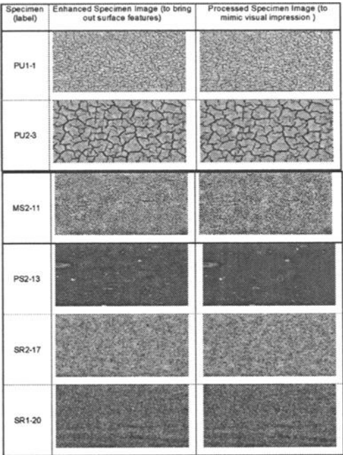
FIG. 9—Enhanced and processed images of weathered sealant surfaces.
