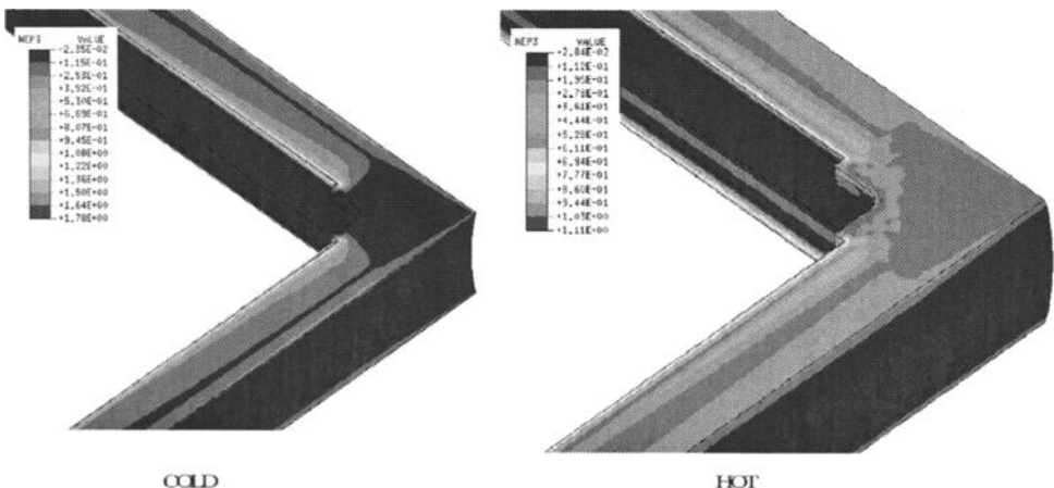
FIG. 7—Nominal strain distribution in edge seal (aluminum spacer, DOW CORNING 982).
