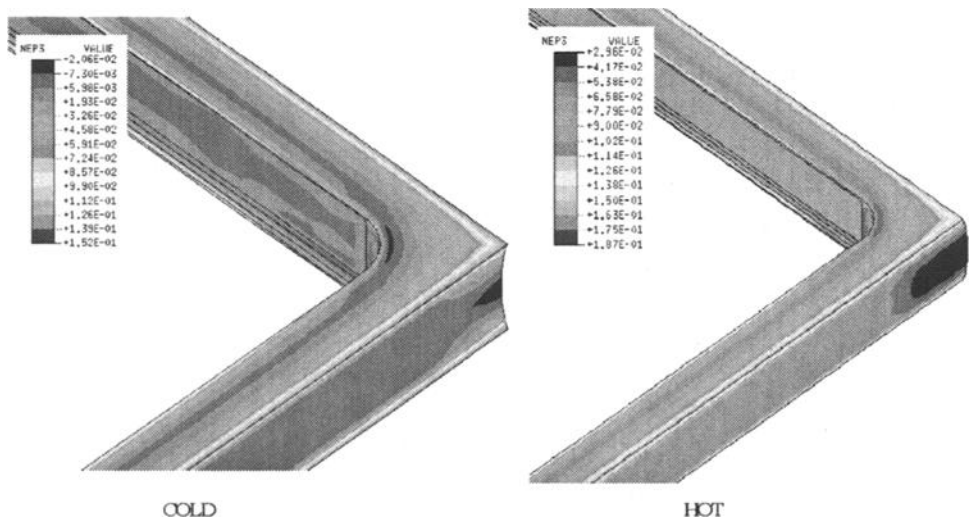
FIG. 9—Nominal strain distribution in edge seal (stainless steel spacer, DOW CORNING 3-0117).
