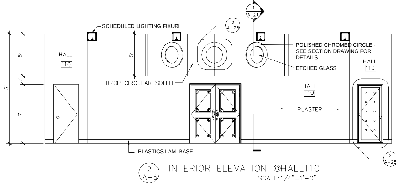
Figure 40. Section and detail symbols shown on an elevation drawing
