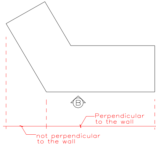
Figure 35. Drawing an elevation drawing for a building in an irregular shape will distort the view.
