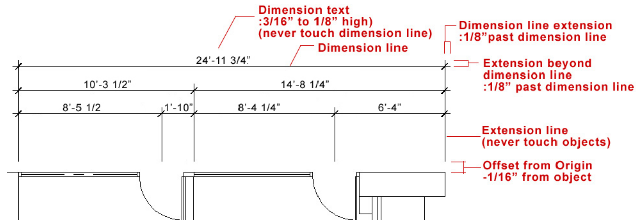
Figure 28. Dimension techniques for floor plans
