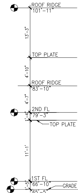
Figure 42. Dimensioning exterior elevations 2
