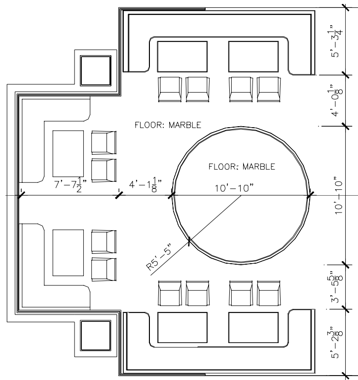
Figure31 Dimensioning a curve
