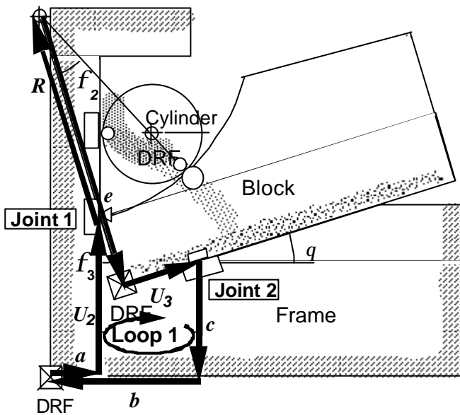
Figure 13-11 Assembly Loop 1
