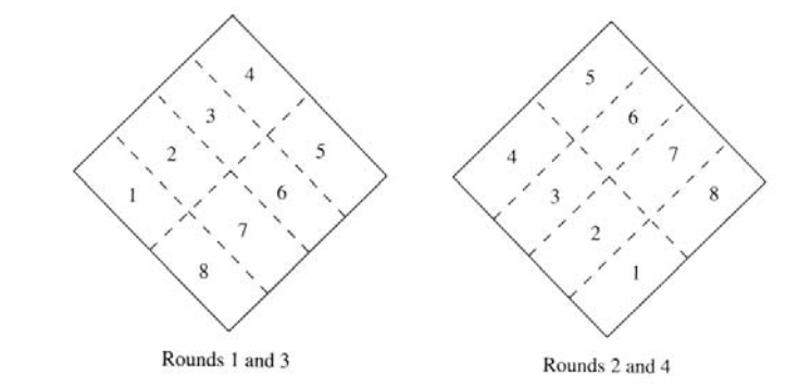
Figure 4 Order of tamping the mortar specimens. (From ASTM. With permission.)
