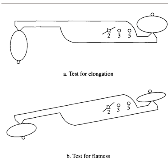
Figure 14 Use of the proportional calipers in testing for particle shape.
