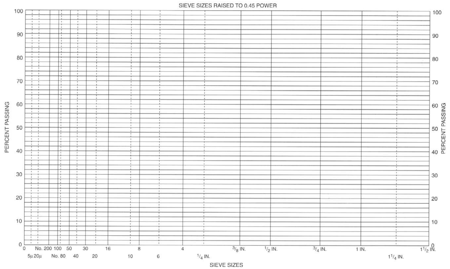
Figure 5c U.S. Bureau of Public Roads 0.45 power gradation chart.
