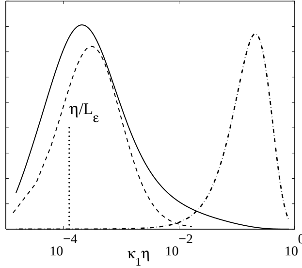
Figure 5.5: One-dimensional pre-multiplied spectra of: — , energy spectrum, \kappa_1 E_{11}(\kappa_1) . ---- , dissipation spectrum, \kappa_1 G_{11}(\kappa_1) ; —·— , Reynolds-stress cospectrum, -\kappa_1 E_{12}(\kappa_1) . Arbitrary units. The flow is a boundary layer from Saddoughi & Veeravali (1994). The vertical dotted line marks the location of the integral scale.
