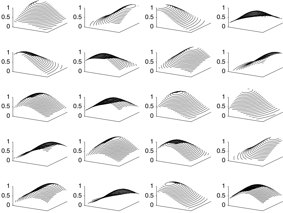
Figure 2.10. The 20 basis functions, with each plot showing the value of \psi^{(i)} within the bounds of the design space \mathbf{D} . At the the centre of the basis function ( \mathbf{x}^{(i)} ) \psi^{(i)} = 1 and as |\mathbf{x}^{(i)} - \mathbf{x}| gets larger the correlation reduces and \psi^{(i)} \rightarrow 0 .
