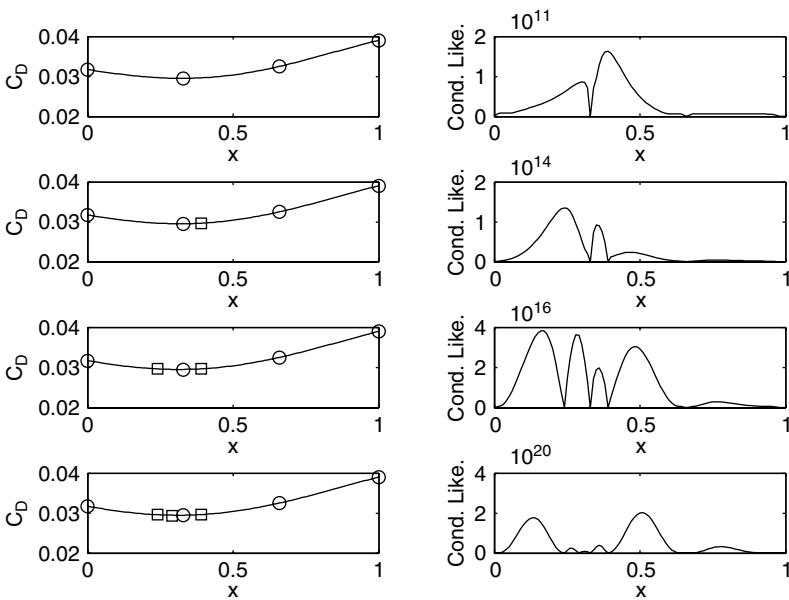
Figure 6.9. A goal seeking search of the aerofoil problem using re-interpolation.
